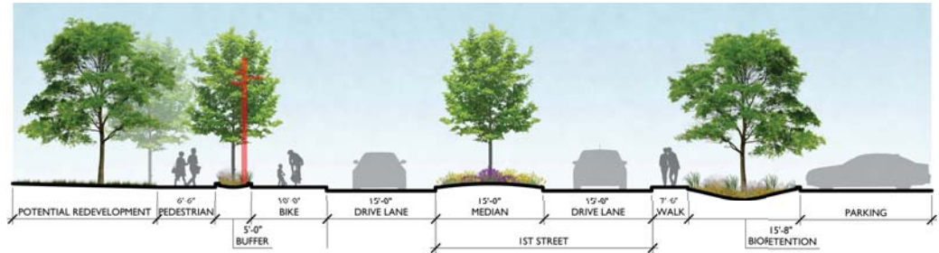
Connect Room Typical Cross Section
