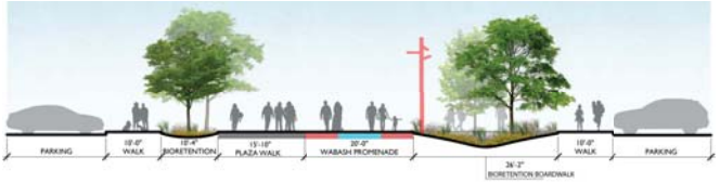
B Gather Room Green Infrastructure Cross Section
