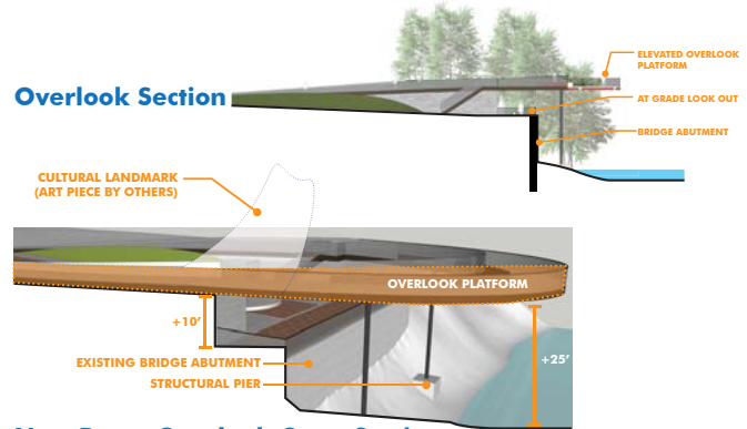
Nest Room Overlook Cross Section
